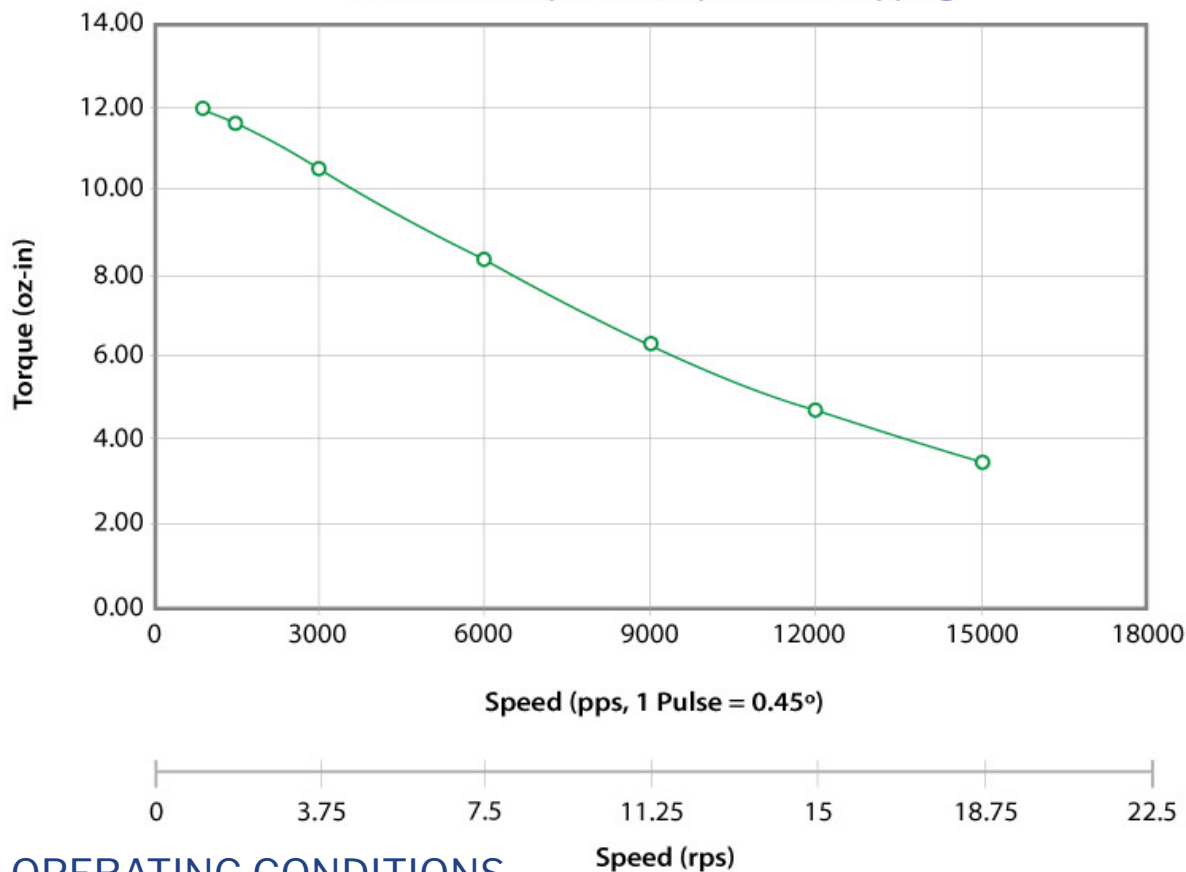
ZH417-11-18 (0.9° Step Motor) 24VDC, 0.6 Amp/Phase, Bipolar, 1/2 Stepping
